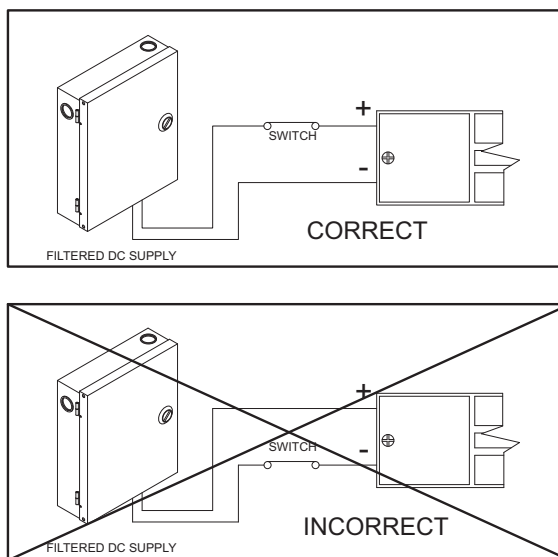
Fig. 2 – Power Connections
